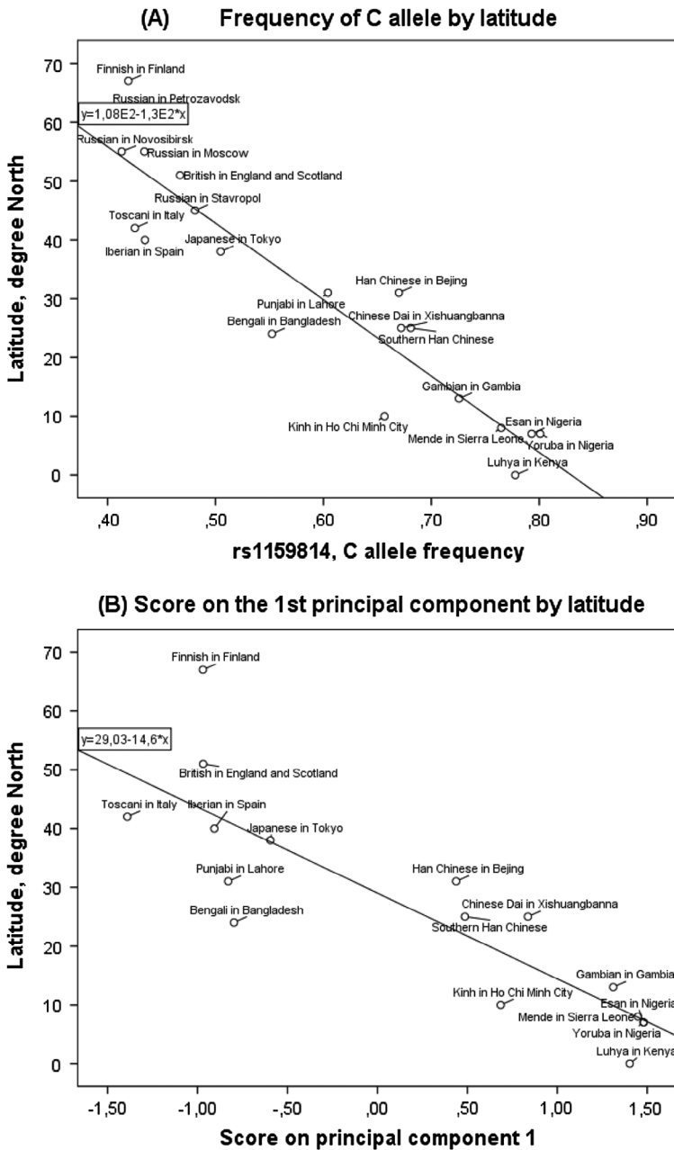
Figure 4. Latitudinal clines of major allele frequency. (A) Major allele frequency for polymorphism in RORα was calculated for each of 20 samples (including 4 Russian samples). Spearman coefficient of correlation attained the values of -0.911 and -0.928 for samples from 16 and 20 populations, respectively ( p < 0.001 for both). (B) Score on the 1st principal component of 7 major allele frequencies was obtained by principal component analysis of samples from 16 African and Eurasian populations of the 1000 Genomes Project Phase 3.
